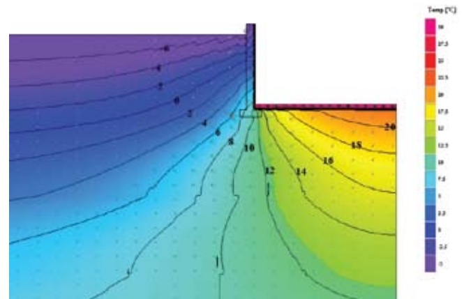
Insulated Slab in February
