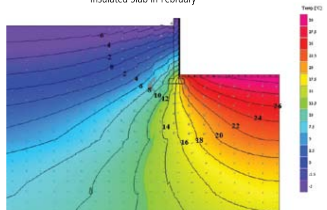
Uninsulated Slab in February
